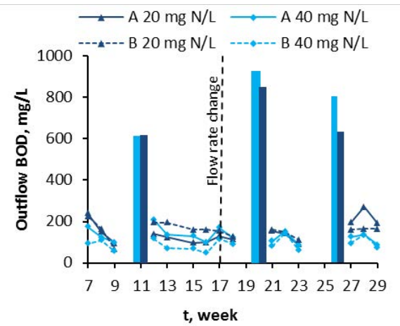
Figure 6 Outflow BOD
