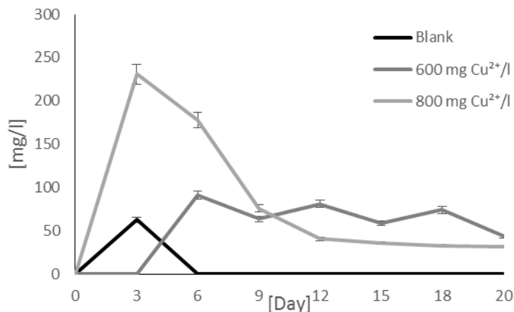
Figure 6 Propionic acid content in sludge
