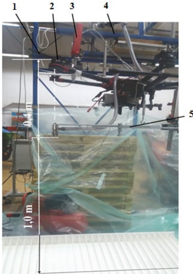
Figure 1 Test station
