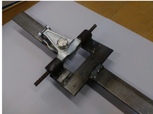
Figure 2 Tested clamp inserted into clamping device
