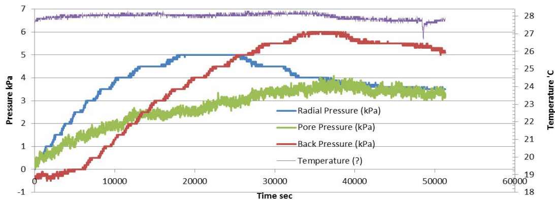
Figure 6 Relationship between the temperature and the back, radial and pore water pressure transducer readings, at the constant laboratory room temperature
